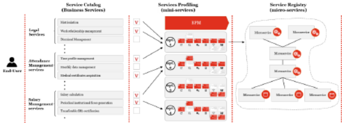
Figure 5. Service, Mini-service, Micro-service
